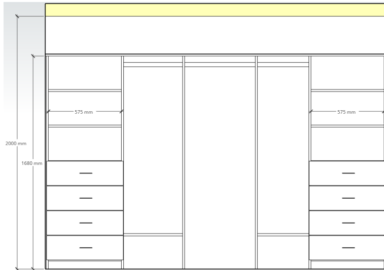
DELUXE Interior #1 - 1700 mm H x 450 mm D. Suitable for opening width > 2440 mm and < 3610 mm
