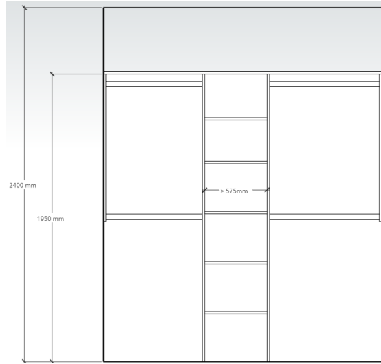
BASIC Interior #2 - 1966 mm H x 450 mm D
