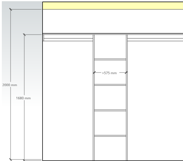
BASIC Interior #1 - 1700 mm H x 450 mm D
