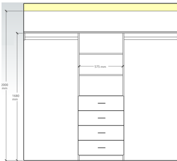
STANDARD Interior #1 - 1700 mm H x 450 mm D
