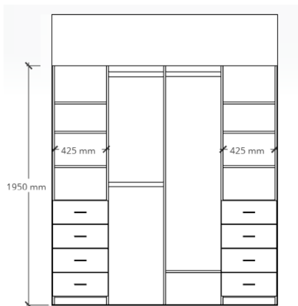
DELUXE Interior #2 – 1966 mm H x 450 mm D. Suitable for opening width > 1850 mm and < 2440 mm
