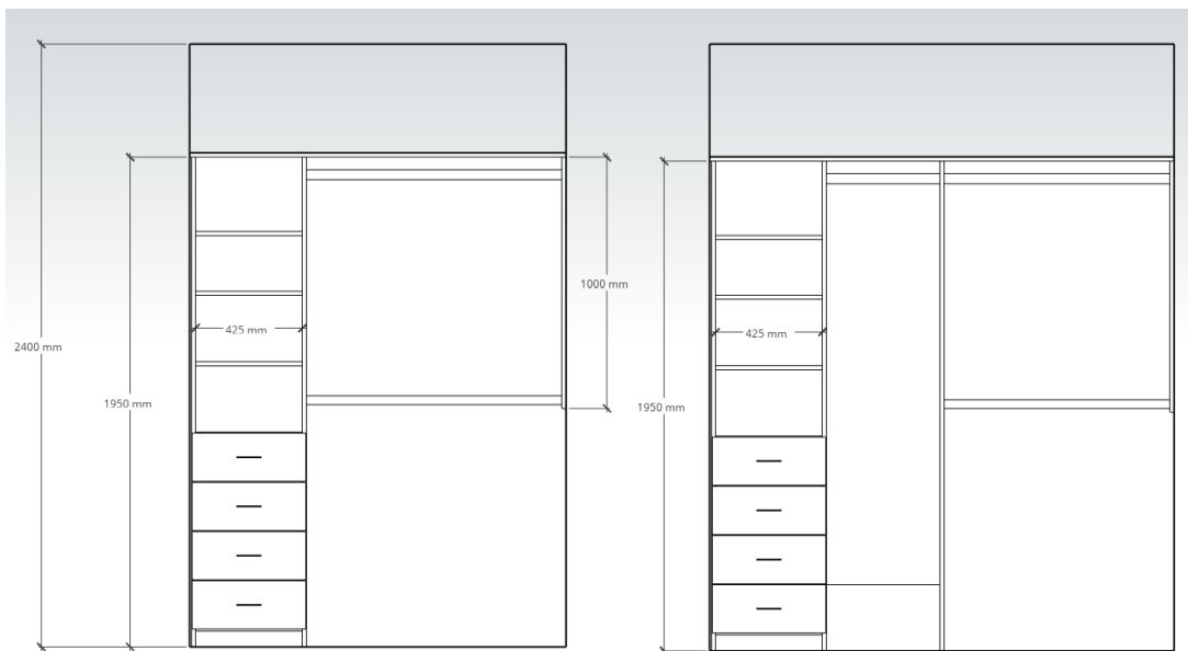
STANDARD Interior #2 - 1966 mm H x 450 mm D. Suitable for opening width > 1150 mm and < 2440 mm
