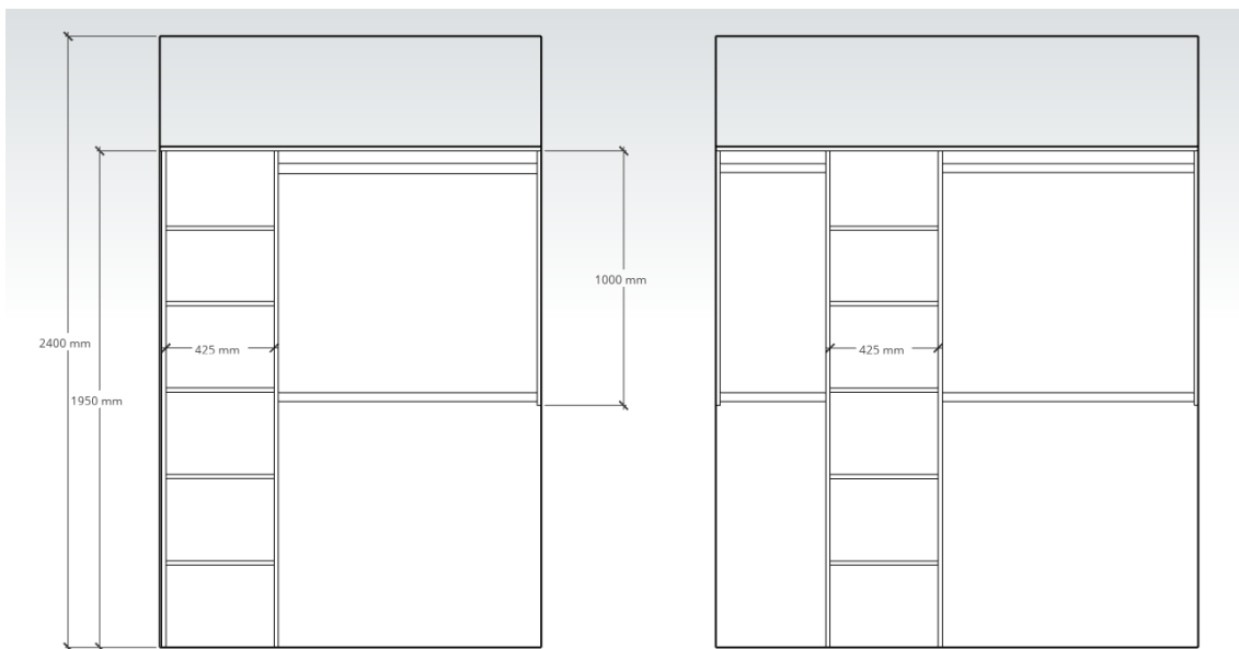
BASIC Interior #2 – 1966 mm H x 450 mm D. Suitable for opening width > 1150 mm and < 2440 mm
