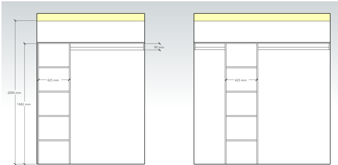
BASIC Interior #1 - 1700 mm H x 450 mm D. Suitable for opening width > 1150 mm and < 2440 mm
