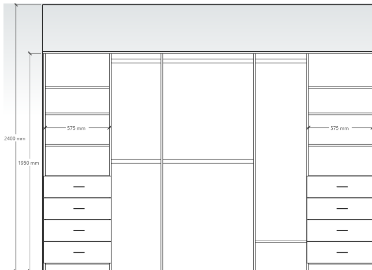
DELUXE Interior #2 – 1966 mm H x 450 mm D. Suitable for opening width > 2440 mm and < 3610 mm
