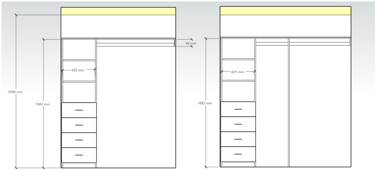
STANDARD Interior #1 - 1700 mm H x 450 mm D. Suitable for opening width > 1150 mm and < 2440 mm
